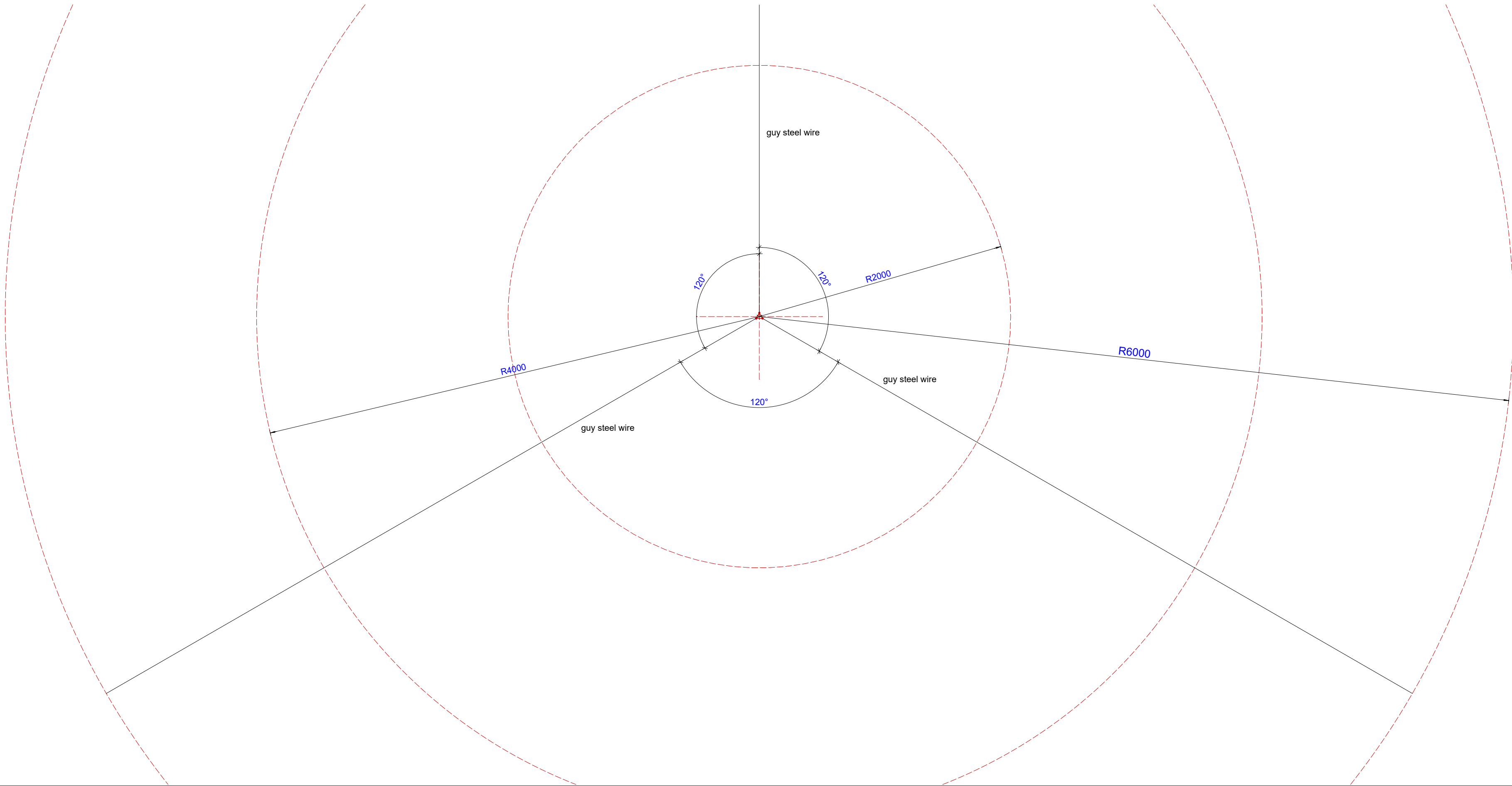
Guy wire and anchors positioning plan 1:250
