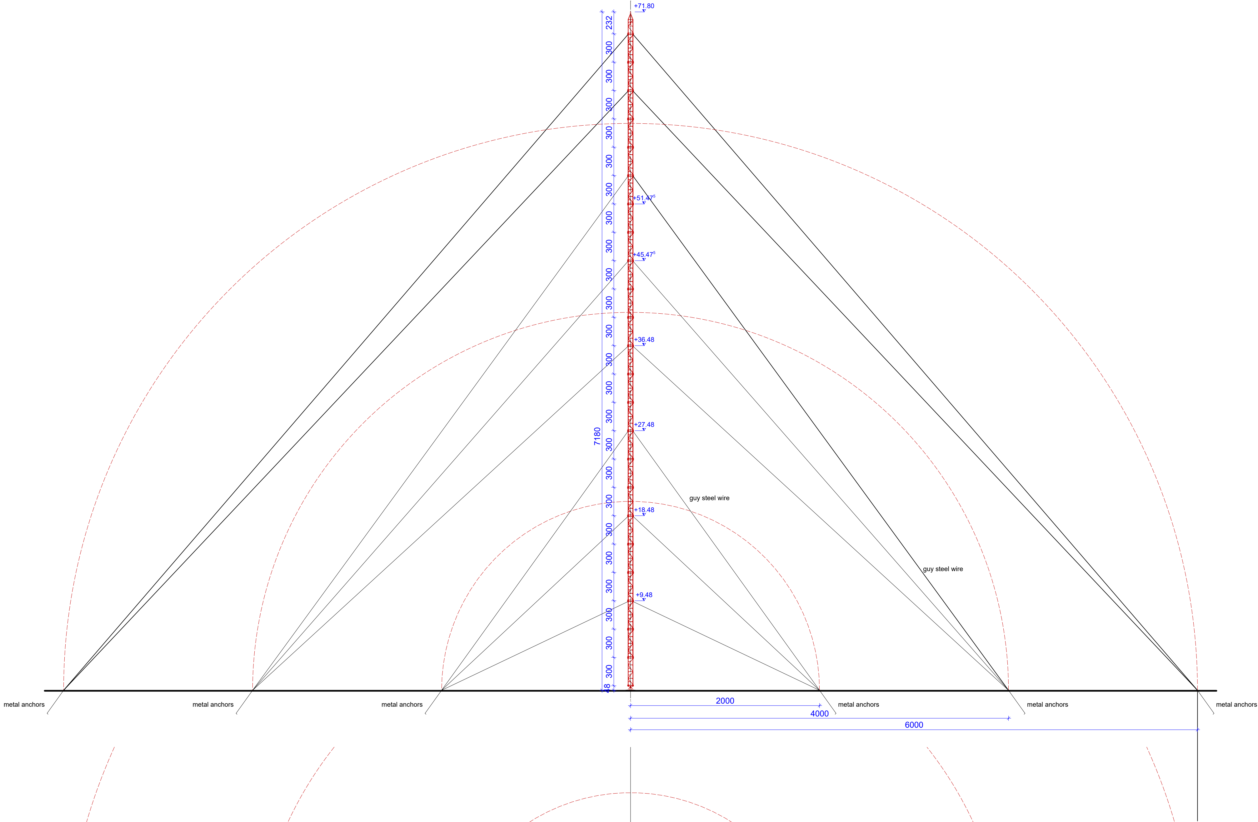
Mast Elevation 1:250
